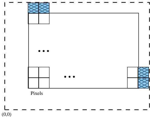
Frame: luma
