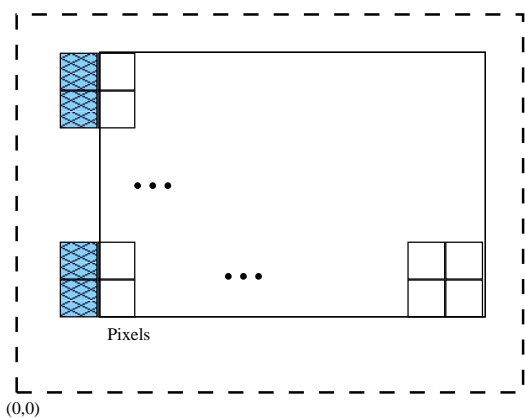
Frame: luma
